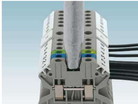
Touch-proof safety Test finger with 12.5 mm diameter
