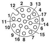
Female, 17-pos.
